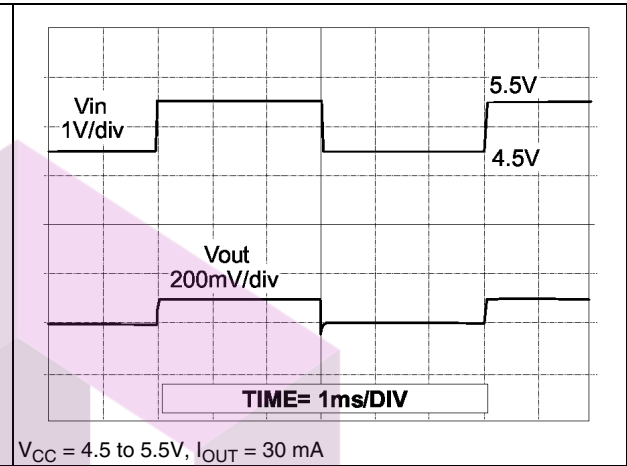
Figure 20. Load transient response ( I_{OUT} = 30\text{ mA} )
